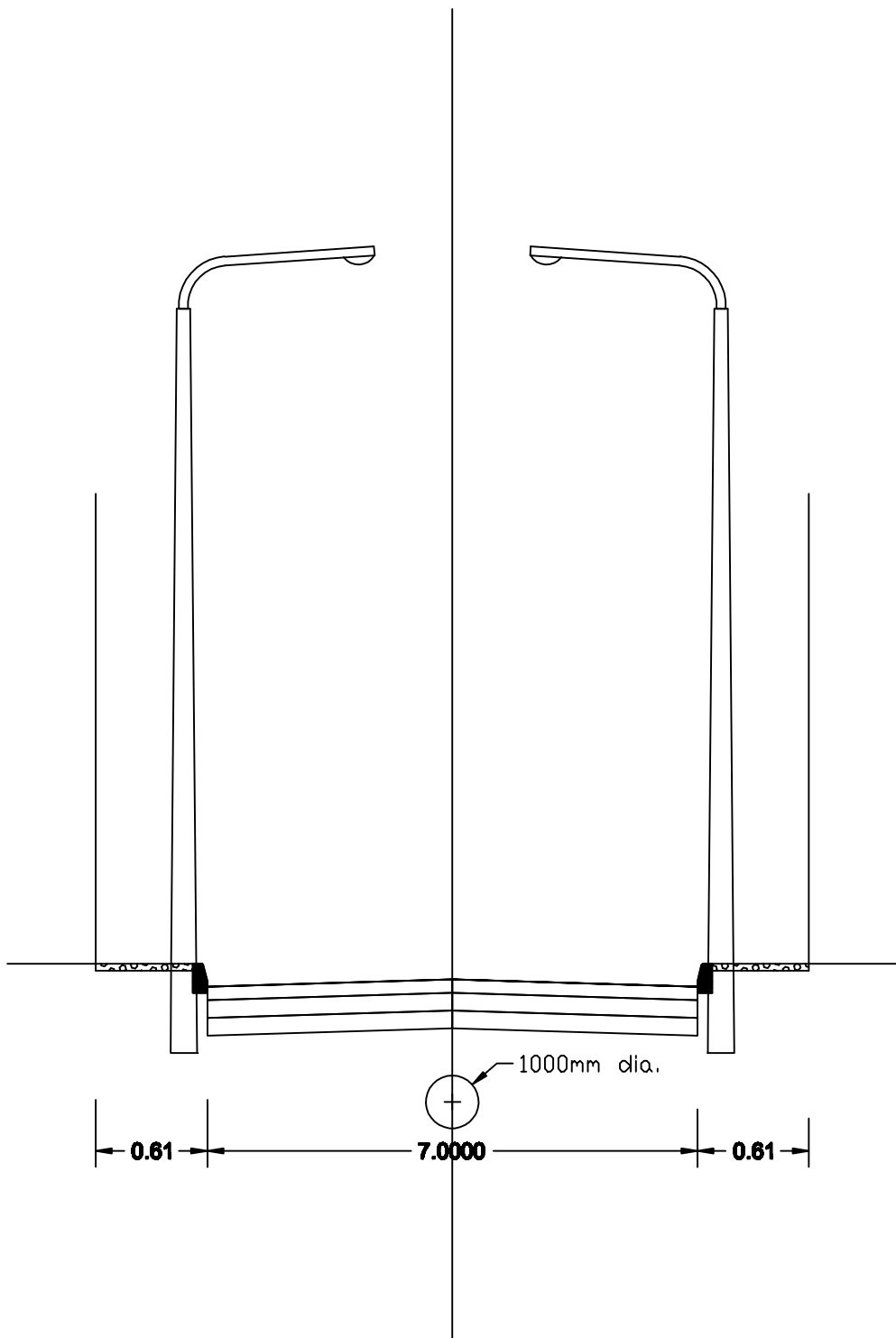
TYPICAL CROSS SECTION OF ROAD For Nepatar Chowk to Phutung (0+000 to 0+146m)
